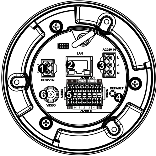
CP-6408-21-I Connectors
