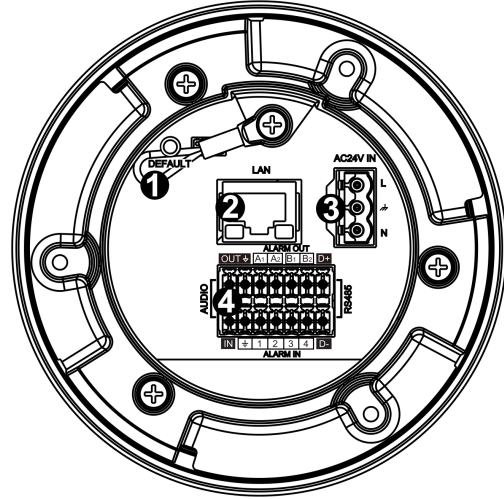
CP-6408-31-I Connectors
