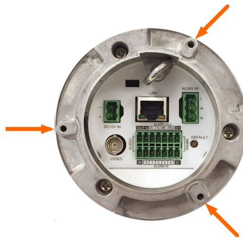
Pendant Cap Screw Holes on Camera (CP-6408-21-I)
